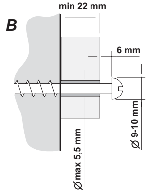
Lower wall distance screw and spacer measures
