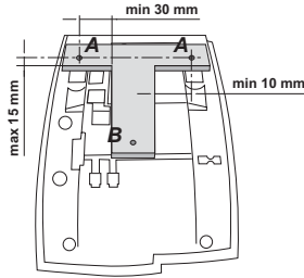
Spacer, alternative 1 (recommended)
