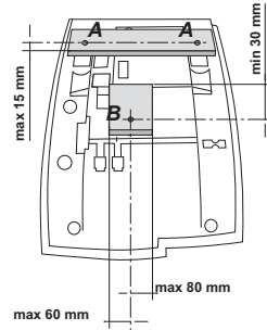
Lower wall distance screw and spacer measures
