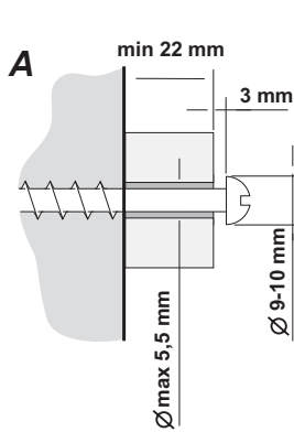
Two upper wall distance screws and spacer(s) measures
